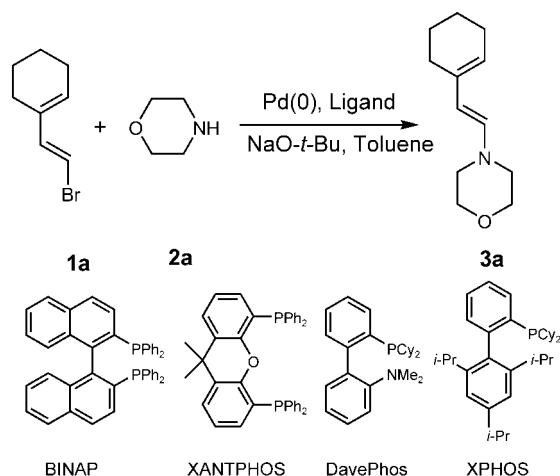
Scheme 1. Coupling reaction of bromodiene 1a and morpholine 2a under different catalytic conditions.
